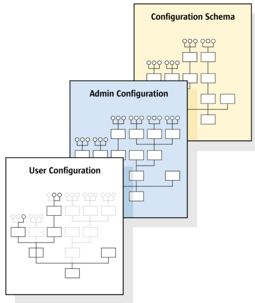
Configuration layers
