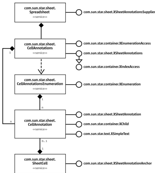
Cell annotations
