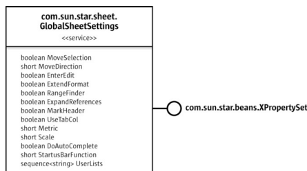
GlobalSheetSettings
