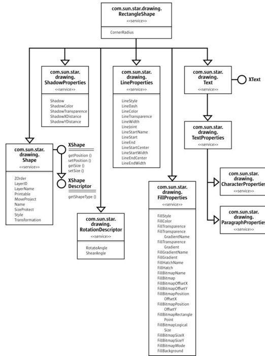
RectangleShape
