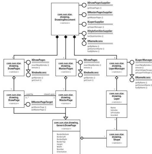
DrawingDocument Structure
