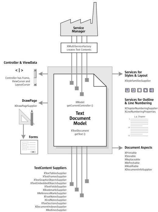
Text Document Model
