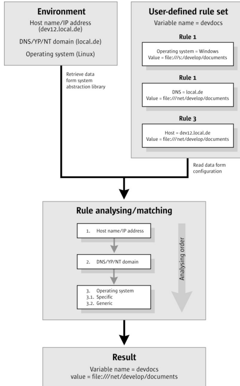
Process of the rule set analyzing
