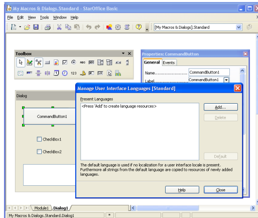
Dialog Editor with Manage User Interface Languages dialog
