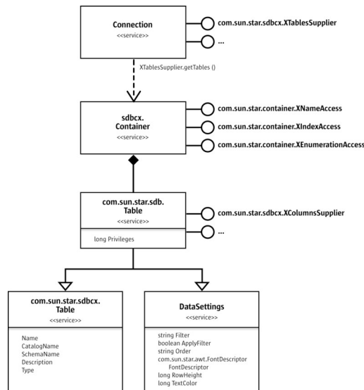
Connection and Tables
