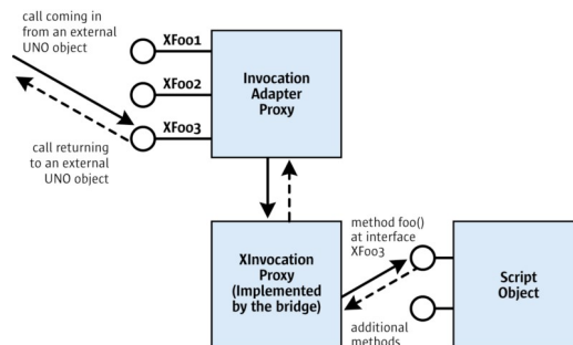
A call sequence
