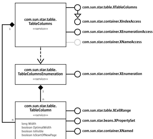
Collection of table columns
