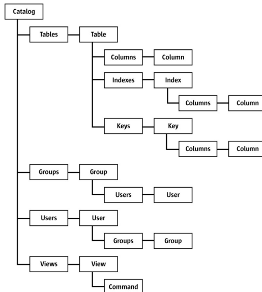
SDBCX Object design
