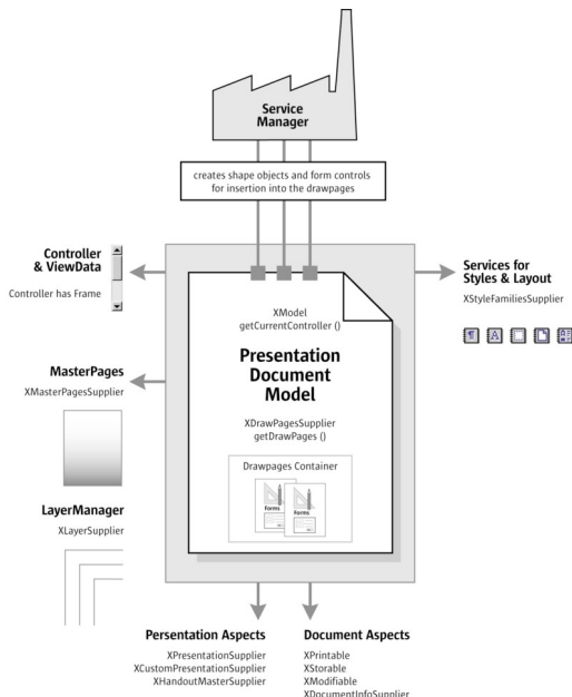
Presentation Document Overview
