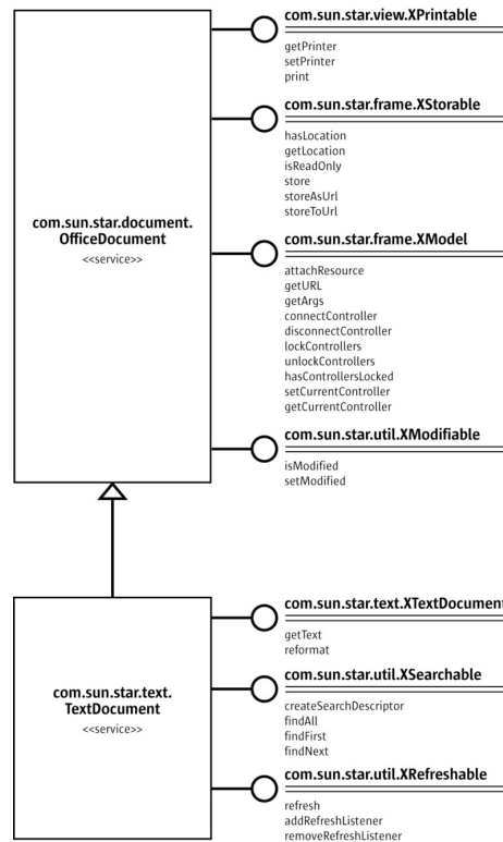
Figure. TextDocument inherits the methods of OfficeDocument.
