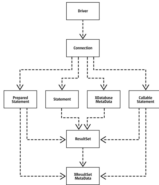
Dependency between driver classes
