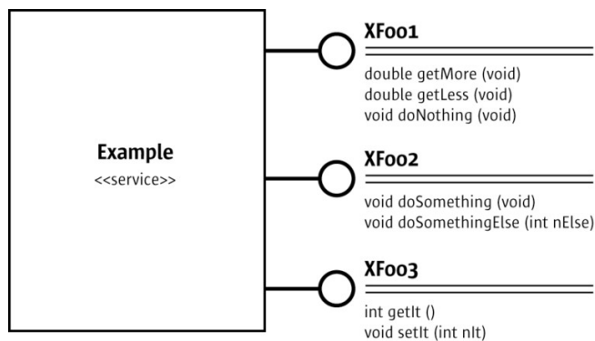
Basic Hides Interfaces
