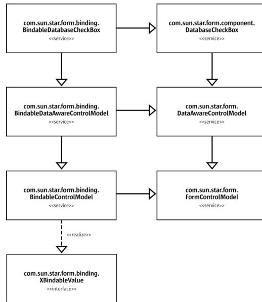
Form control models supporting value bindings
