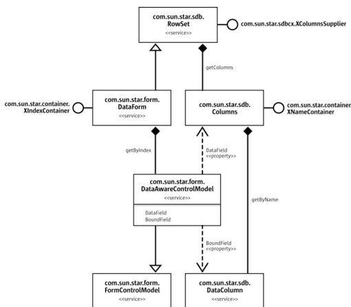
Data awareness relationship
