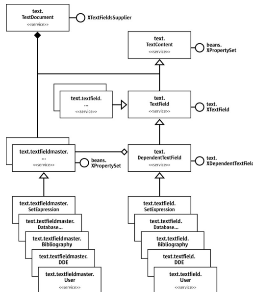
Text Fields and Text Field Masters
