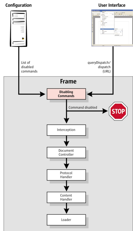
How the disable commands feature works
