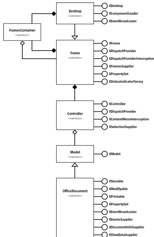
Desktop Service and Component Framework
