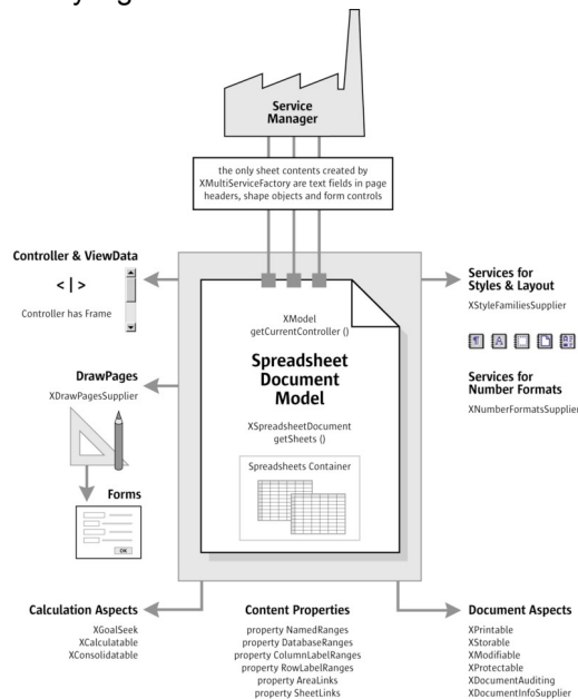
Spreadsheet Document Component
