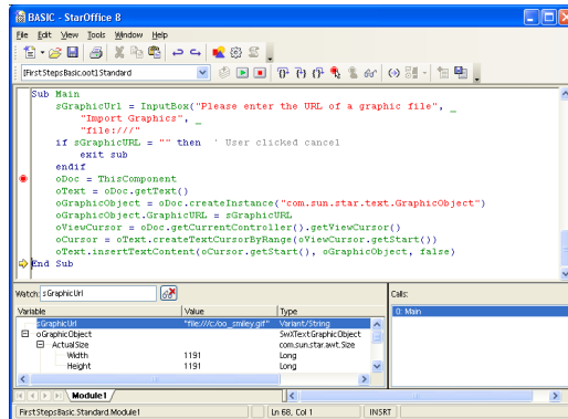
A macro in the source editor window
