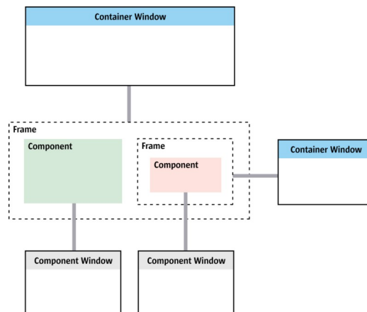
Frame containing a component and a sub-frame
