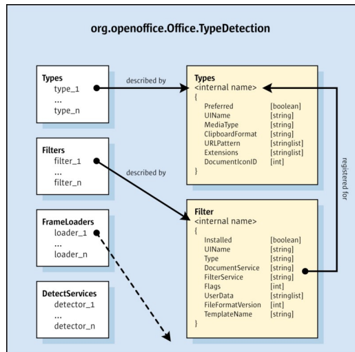
Structure of org.openoffice.Office.TypeDetection Configuration Branch
