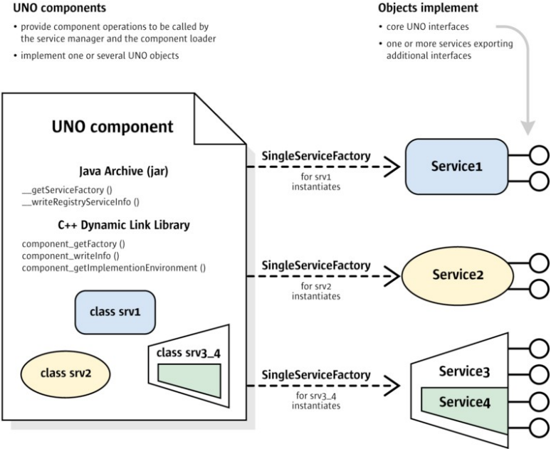
A Component implementing three UNO objects
