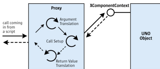
A scripting call over a proxy instance
