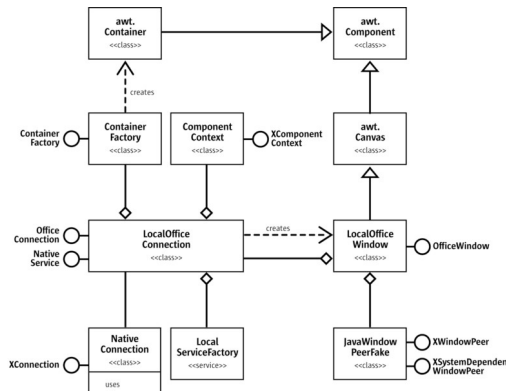
The OfficeBean structure
