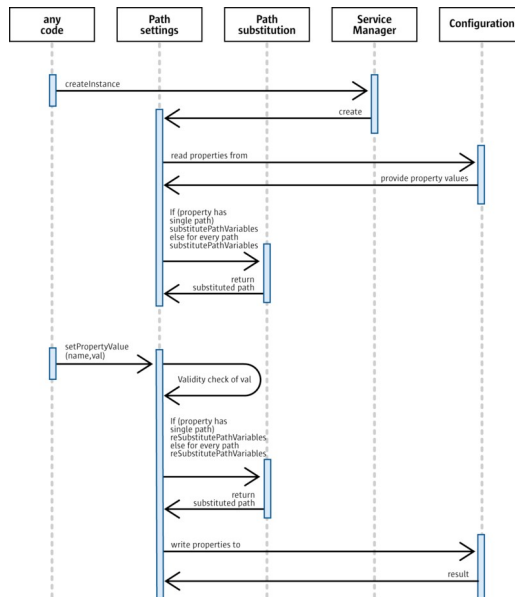
Interaction of path settings, path substitution and configuration
