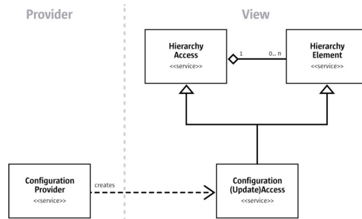
Configuration object model overview
