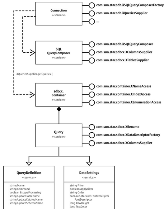
Connection, QueryComposer And Query in the sdb Module
