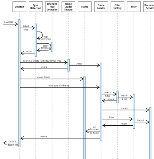
General Filtering Process
