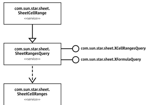
Query sheet ranges
