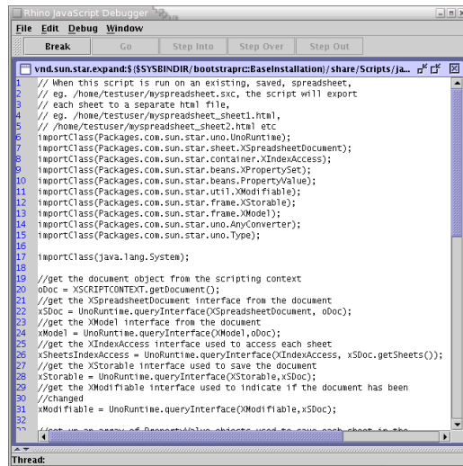
JavaScript Debugger
