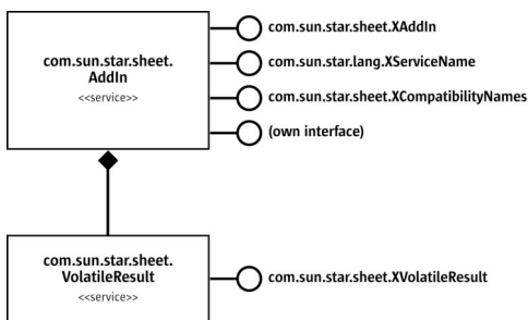
AddIn
