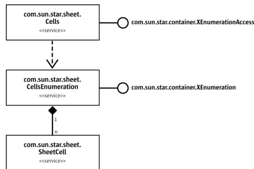
Cell collections
