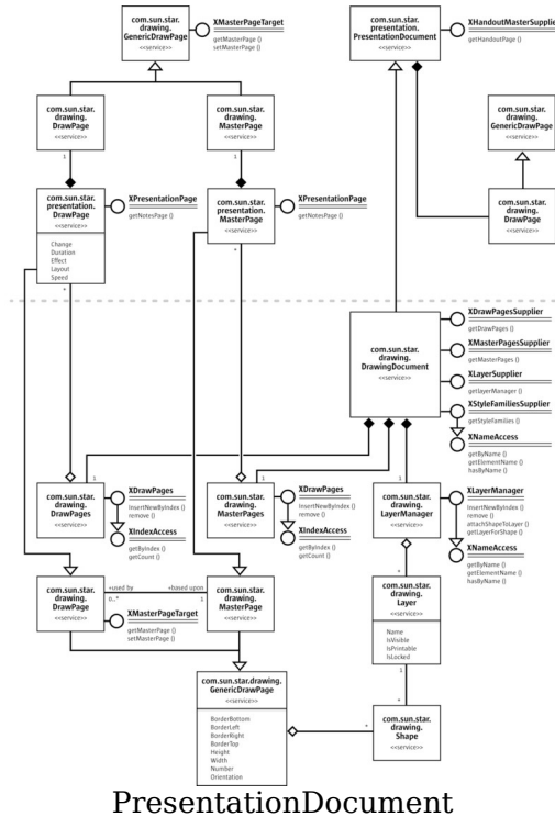
PresentationDocument
