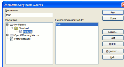
Macro dialog
