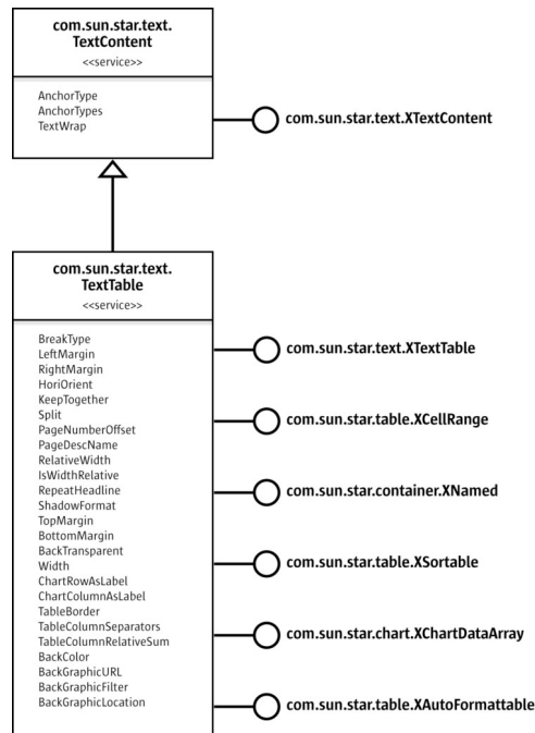
Service com.sun.star.text.TextTable
