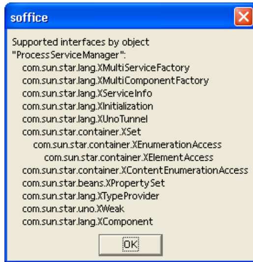
Dbg_SupportedInterfaces Property
