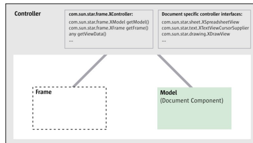
Controller with Model and Frame
