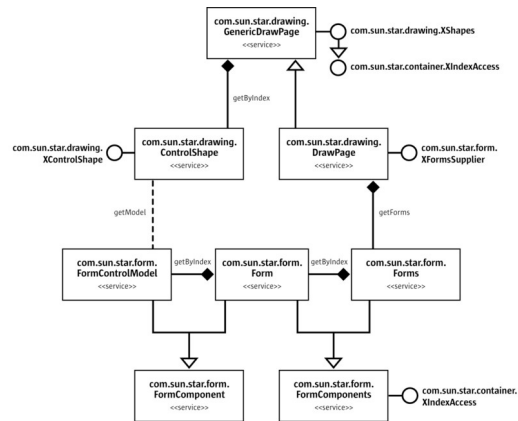
A complete object structure
