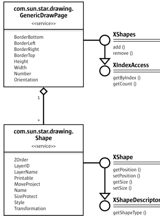
Shape
