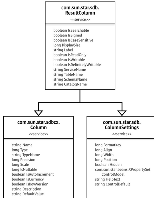
ResultColumn
