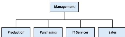
Sample Organigram
