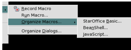
Tools-Macros submenu
