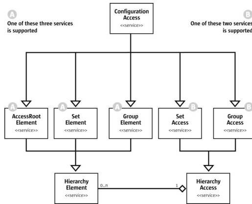
ConfigurationAccess services
