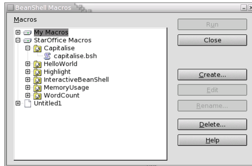
BeanShell Organizer
