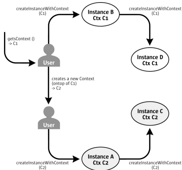
Context propagation.
