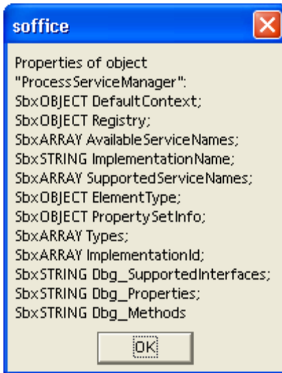
Dbg_Properties
