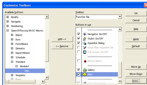
Customize Toolbars
