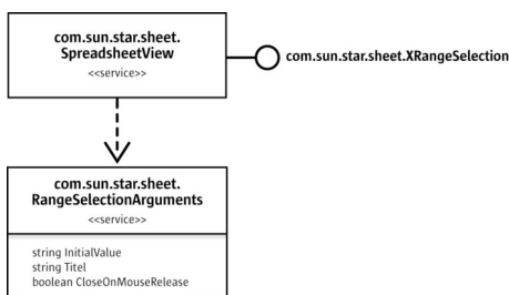
XRangeSelection interface
