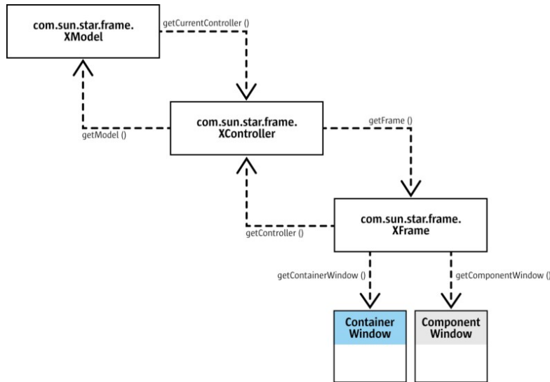
Frame-controller-model organization
