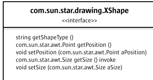
XShape
