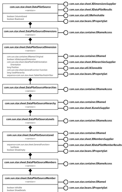
DataPilotSource
