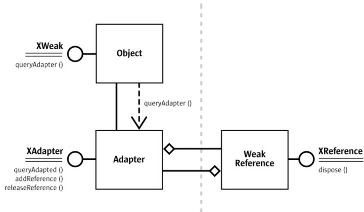
The UNO weak reference mechanism
