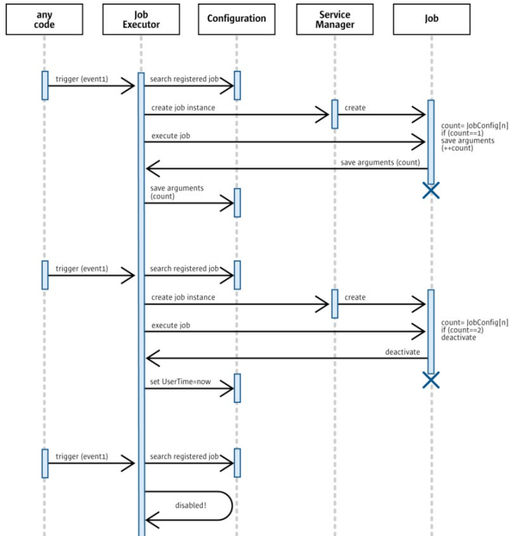
Flow diagram of an example job
