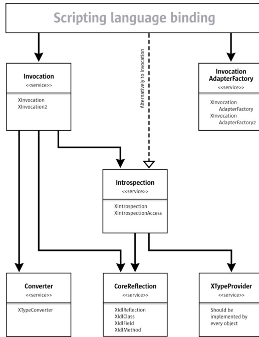
UML diagram showing the a Scripting Language Binding
