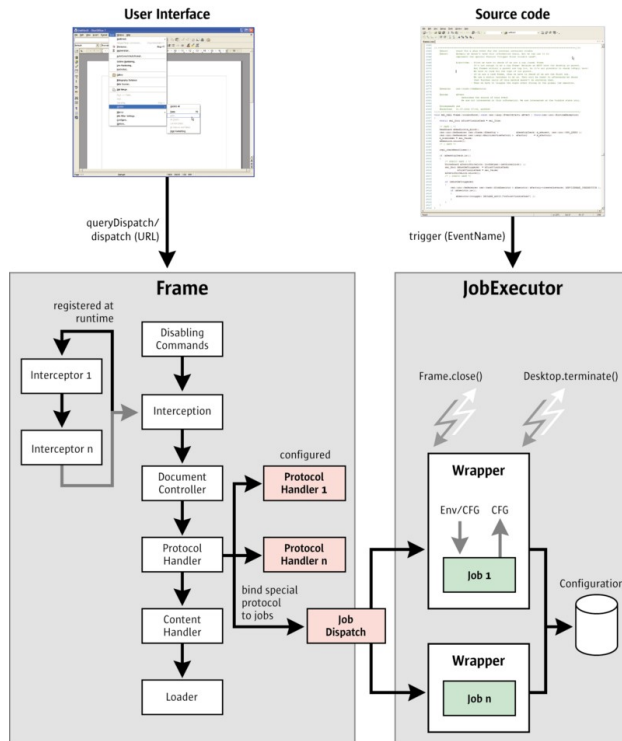
Processing command URLs and the job execution environment
